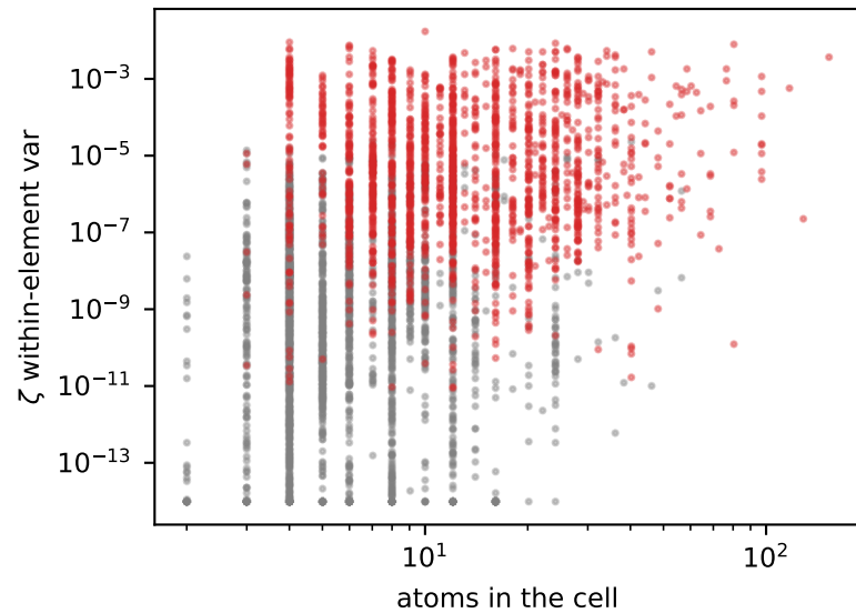
The within-element variance against cell size: a symmetry noise floor (grey) and genuine site differences (red)
