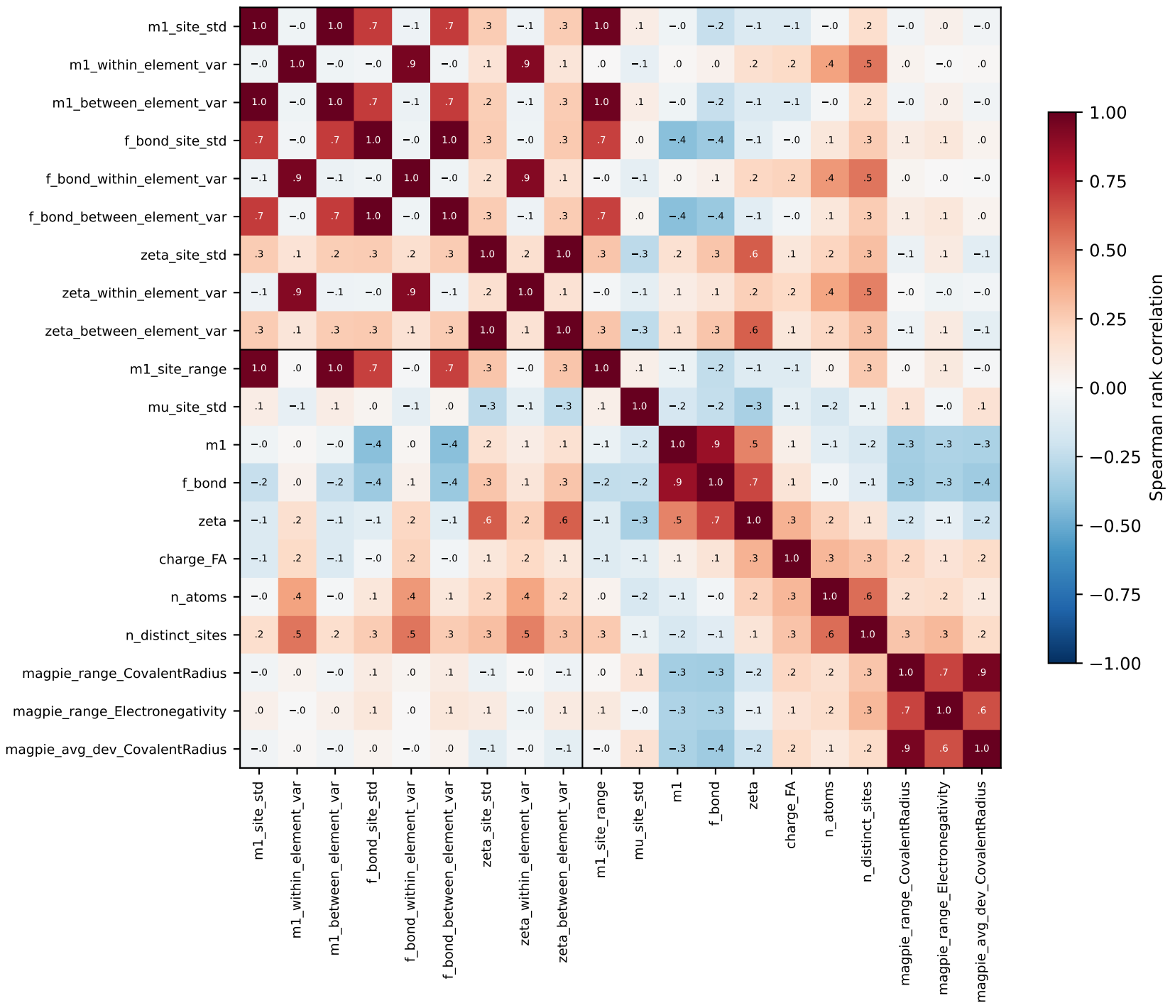
Rank correlations over the 6,059 structures (pairwise complete)
