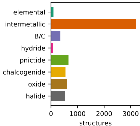
(b) chemical classes
