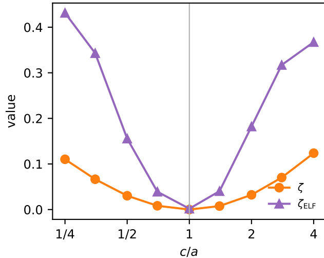
(b) anisotropic Gaussian: \zeta
