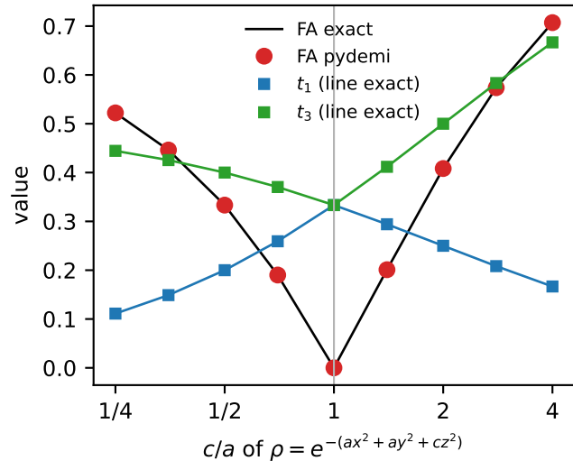
(a) anisotropic Gaussian: tensor
