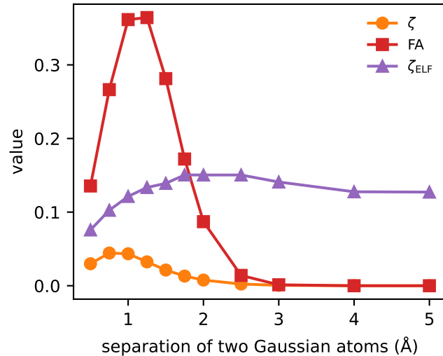
(c) two atoms merging
