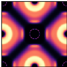
NaCl (ionic) \zeta_{\text{ELF}} = 0.235
