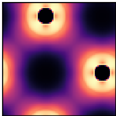
Si (covalent) \zeta_{\text{ELF}} = 0.140
