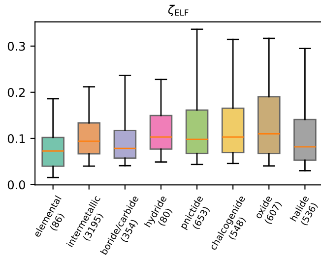
Distributions by chemical class (box: quartiles, whiskers: 5th-95th percentile)
