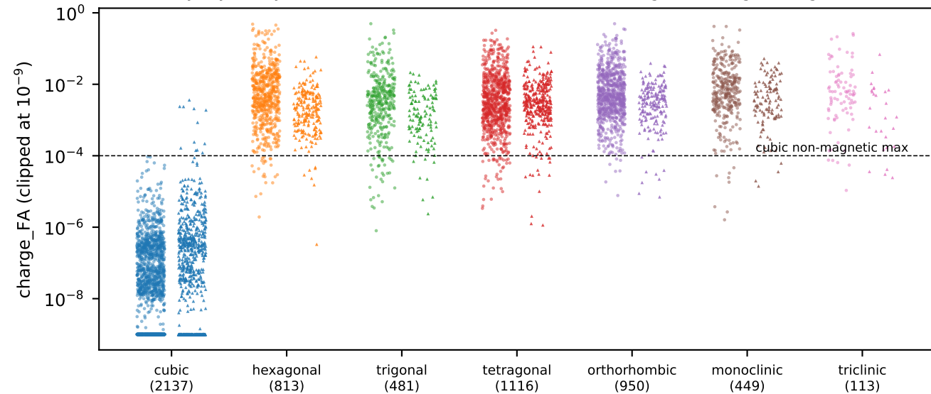
(a) by crystal system of the relaxed structure (left: non-magnetic o, right: magnetic ^)
