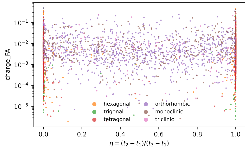
(a) tensor shape (structures with t_3 - t_1 > 10^{-6} )
