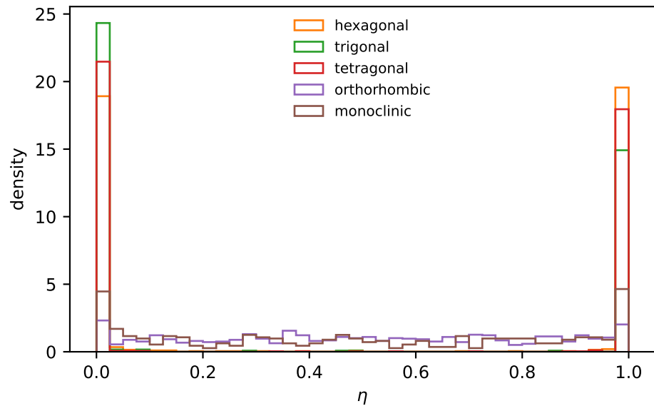
(b) uniaxial systems sit at \eta = 0 or 1
