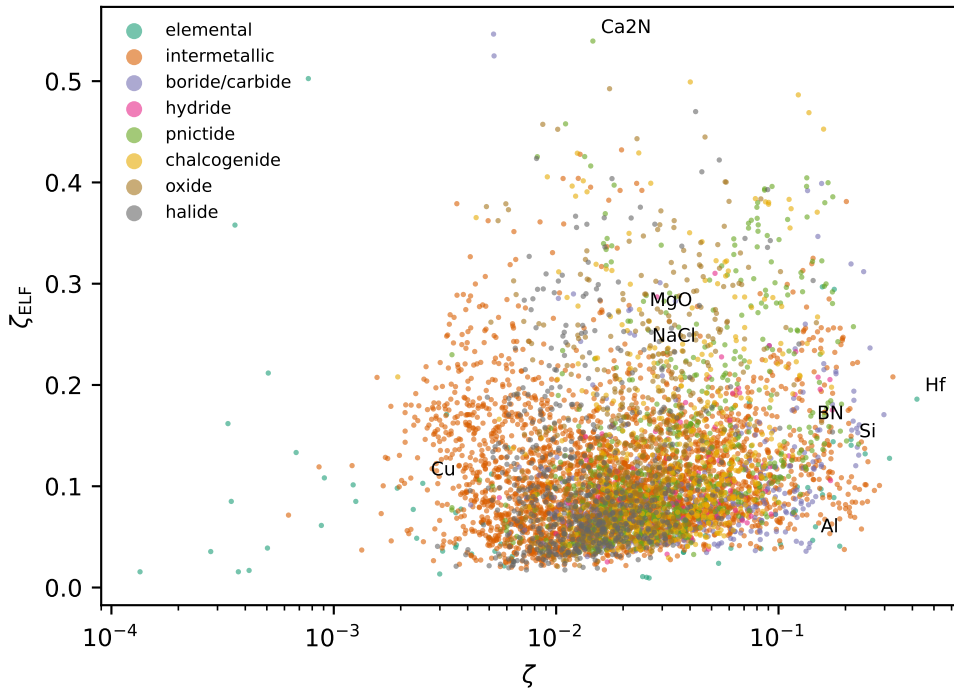
\zeta vs \zeta_{\text{ELF}} (Spearman 0.18)
