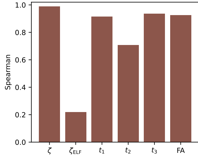
(b) ML density (ChargeE3Net) vs DFT, 605 tests
