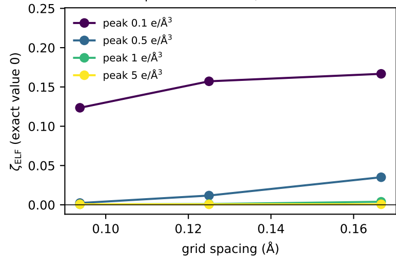
spherical Gaussian, \alpha = 1 \text{ \AA}^{-2}
