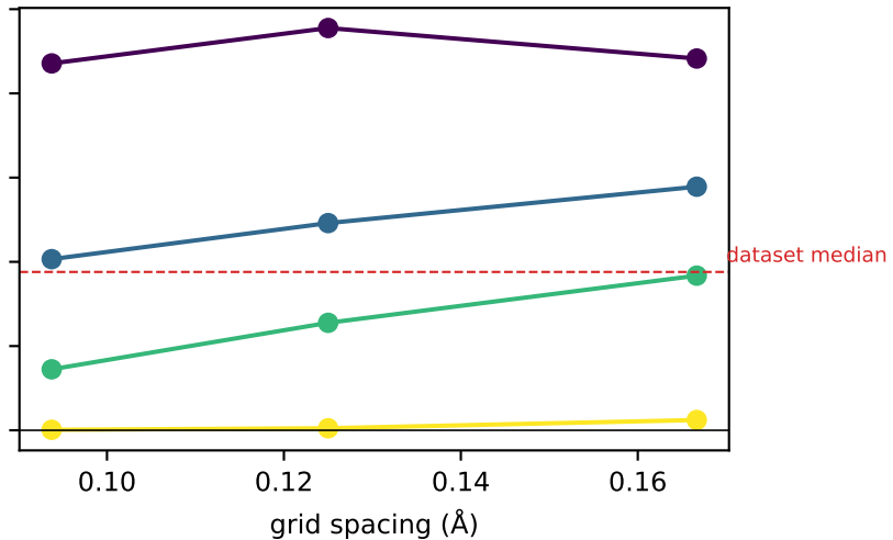
spherical Gaussian, \alpha = 2 \text{ \AA}^{-2}
