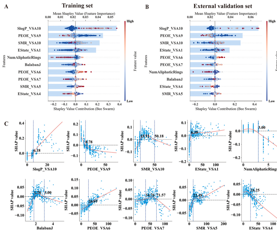
Fig. 4. Global interpretation of molecular features contributing to DIA prediction using SHAP analysis. (A) SHAP summary plot for training set and (B) external validation set showing consistent feature importance patterns across the top 10 molecular descriptors. The x-axis represents the SHAP value contribution (impact on model output), and color indicates the feature value (red for high, blue for low). (C) SHAP dependence plots ordered by the top 10 feature importance from training set, illustrating the relationship between feature values (x-axis) and their impact on model prediction (y-axis), with identified threshold values indicated by vertical dashed lines. The red curves represent LOWESS (Locally Weighted Scatterplot Smoothing) fit to visualize the overall trends. SHAP values higher than zero correspond to a positive class prediction in the model, indicating higher DIA toxicity risk, while negative values suggest lower risk.
