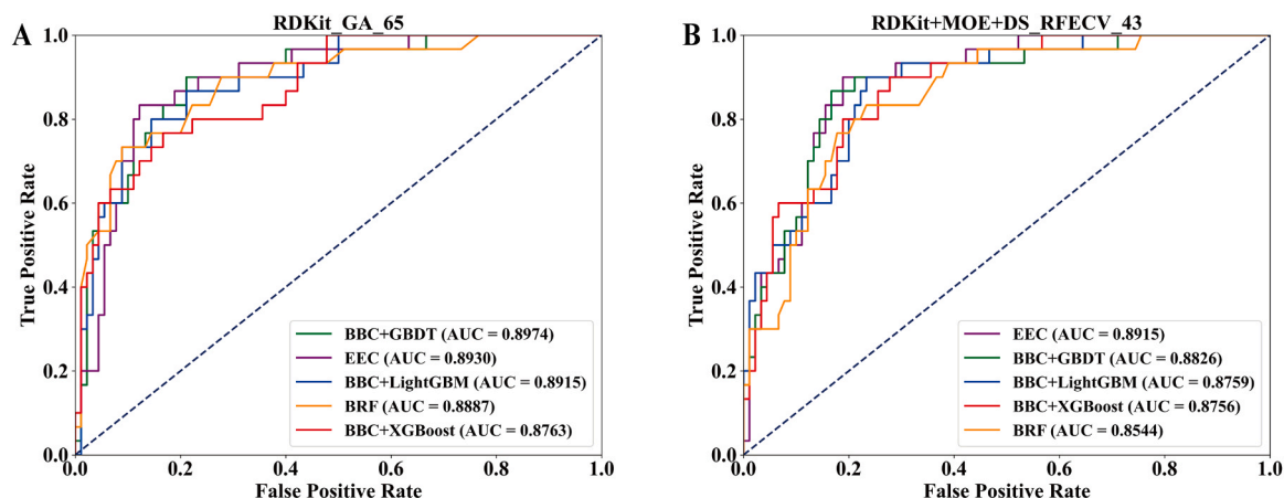
Fig. 2. ROC curves comparing the performance of different ensemble models on the external validation set using (A) RDKit_GA_65 and (B) RDKit+MOE+DS_RFECV_43 feature subsets.
