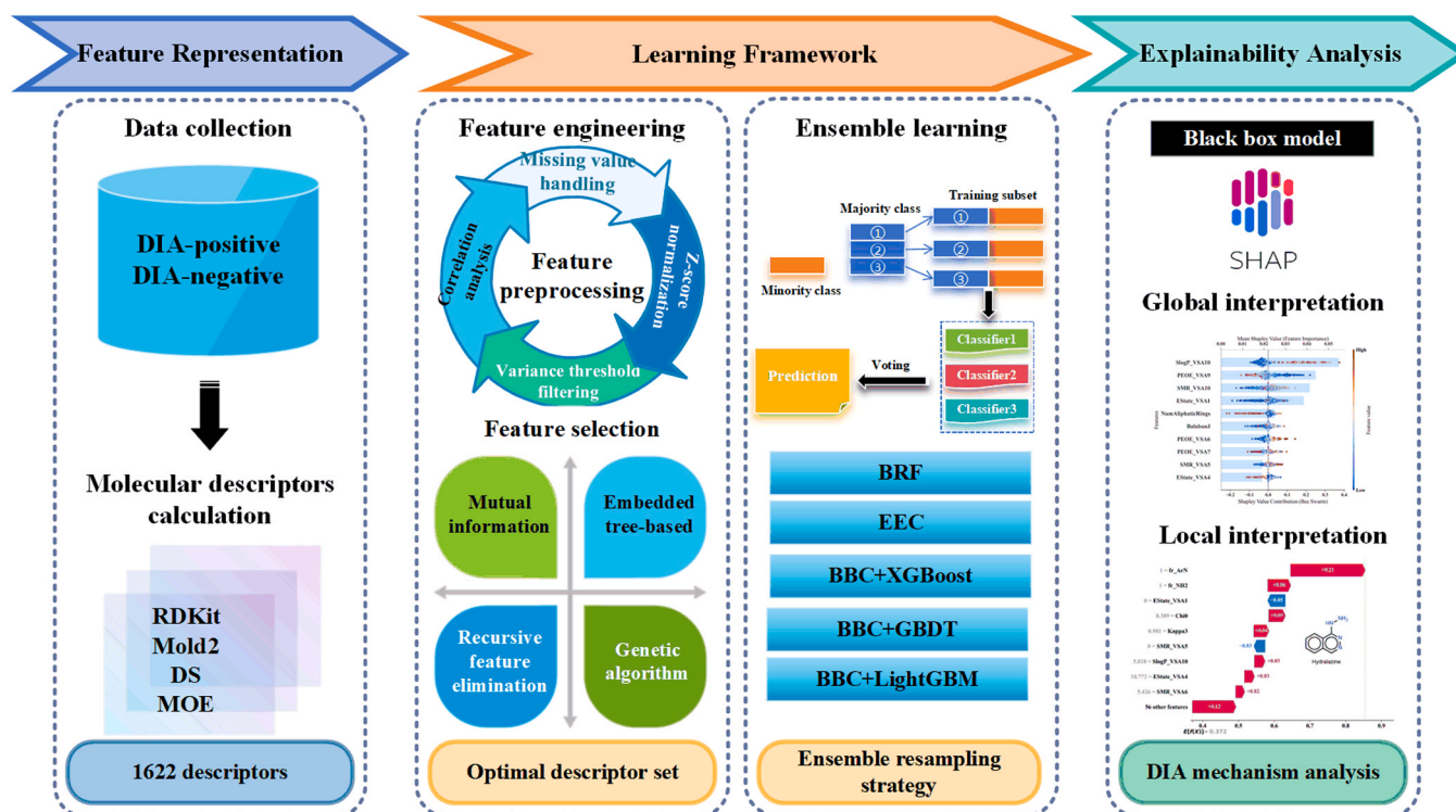
Fig. 1. Schematic illustration of the InterDIA framework for predicting drug-induced autoimmunity.
