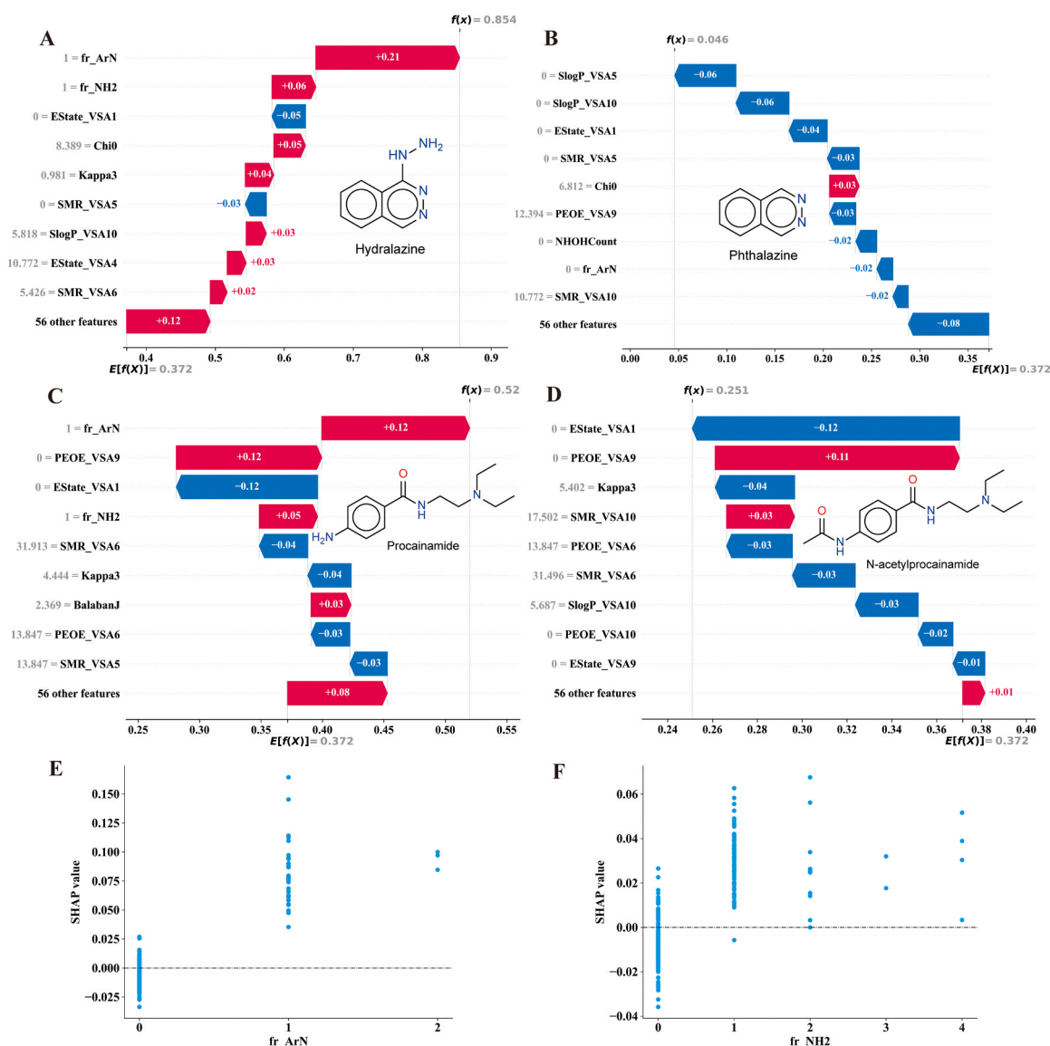
Fig. 5. SHAP analysis of structural features contributing to DIA prediction for drug pairs. (A-D) SHAP waterfall plots showing feature contributions for hydralazine (A), phthalazine (B), procainamide (C), and N-acetylprocainamide (D). Red and blue bars indicate positive and negative contributions to DIA risk, respectively. Chemical features are shown alongside their respective plots. (E-F) SHAP dependence plots for fr\_ArN and fr\_NH2 , demonstrating the relationship between feature presence and their impact on model predictions. The x-axis represents feature values, and the y-axis shows corresponding SHAP values.
