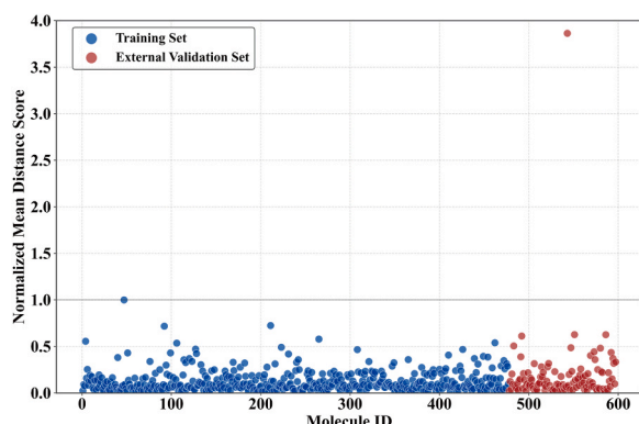
Fig. 3. Applicability domain analysis of the EEC model.
