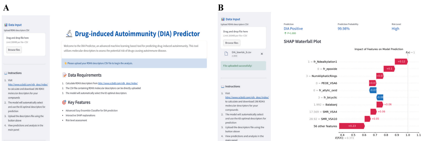
Fig. 6. Online platform for DIA toxicity prediction. (A) Platform homepage demonstrating essential features and input requirements. (B) Example prediction output displaying DIA risk probability and corresponding SHAP waterfall plot illustrating molecular feature contributions to the prediction.
