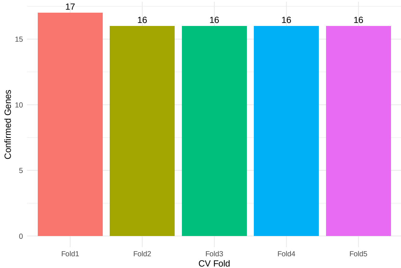
Number of Boruta-Confirmed Genes per CV Fold
