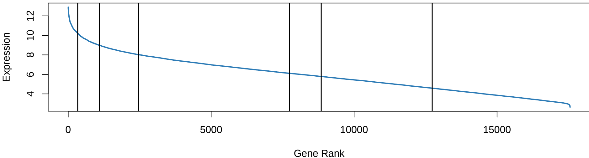
6 Hub Genes ssGSEA Enrichment Curve
