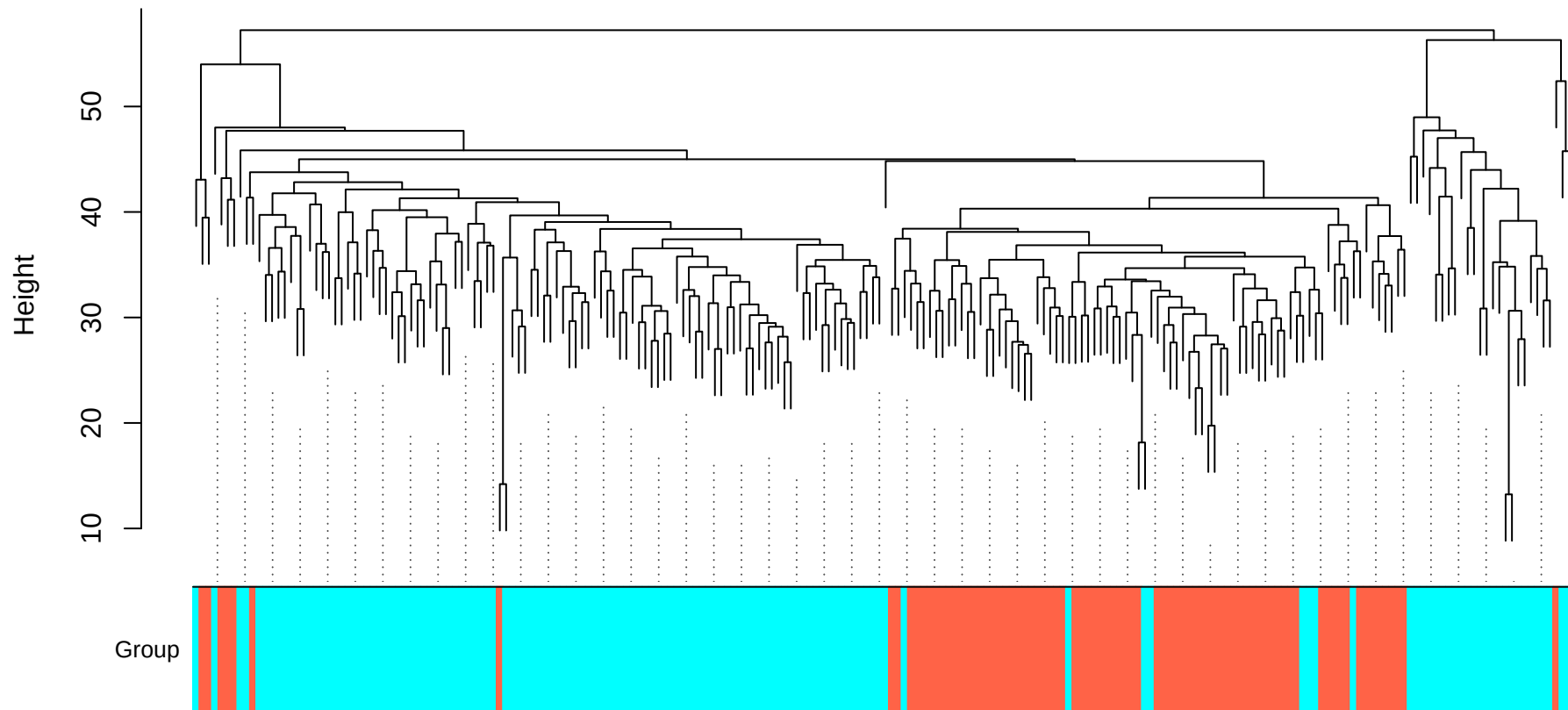
Cluster Dendrogram
