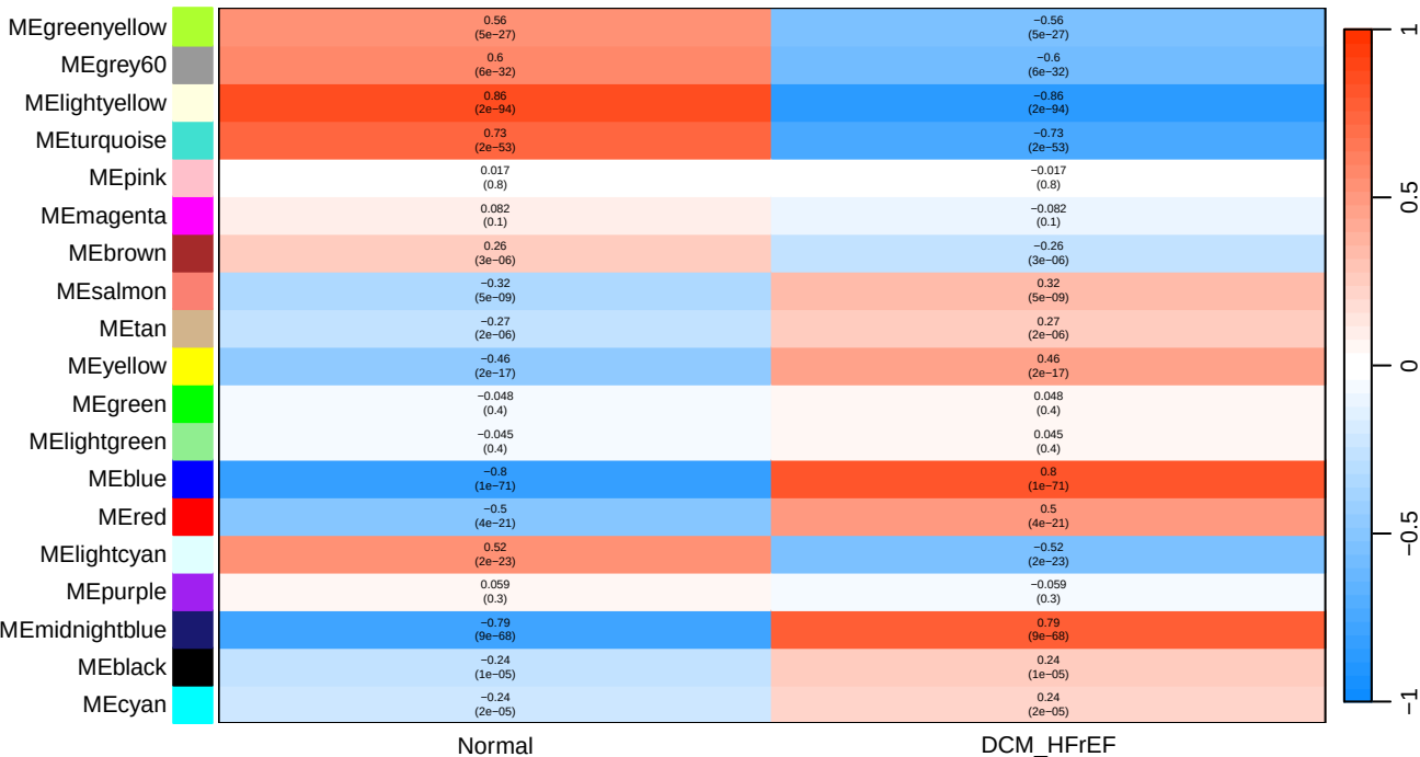
Module-Trait Correlation (DCM-HFrEF vs Normal)
