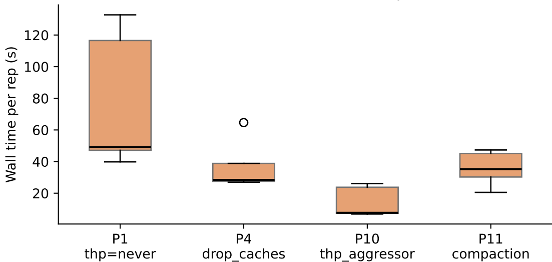
B2 wall-time distribution (5 reps/cell)
