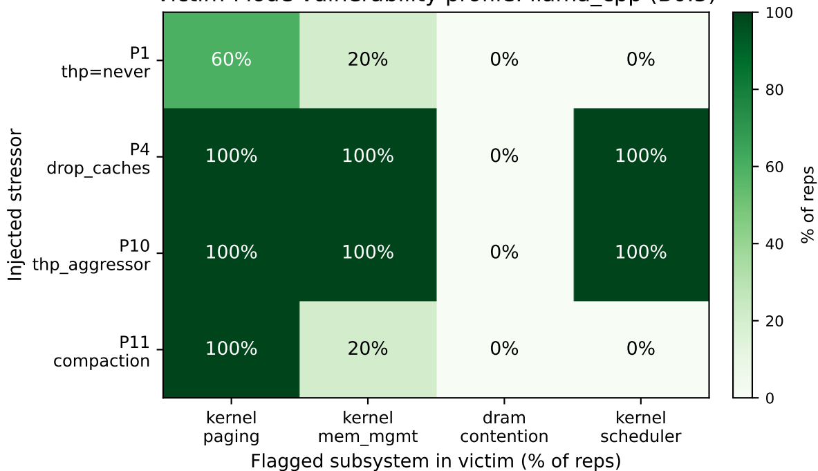
Victim-Mode vulnerability profile: llama_cpp (B0.5)
