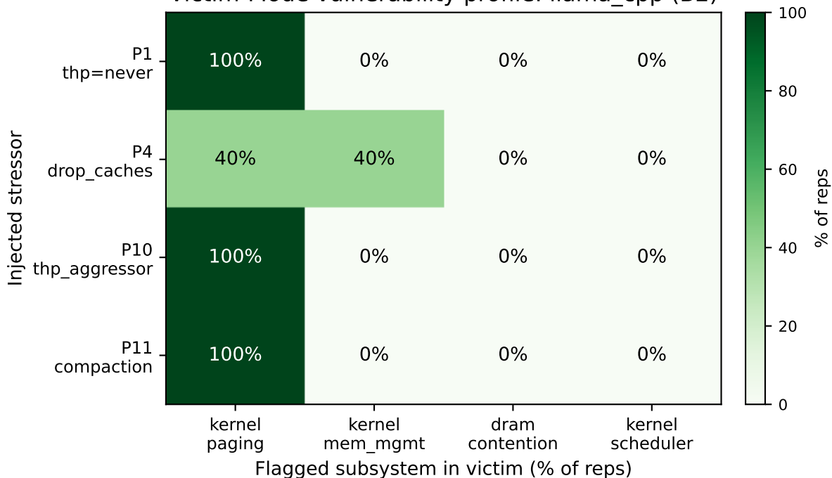
Victim-Mode vulnerability profile: llama_cpp (B2)
