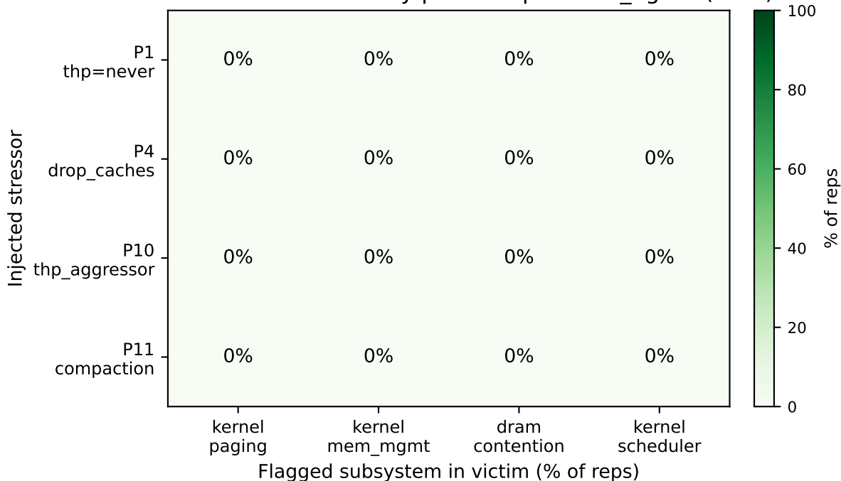
Victim-Mode vulnerability profile: opcode_agent (B0.5)
