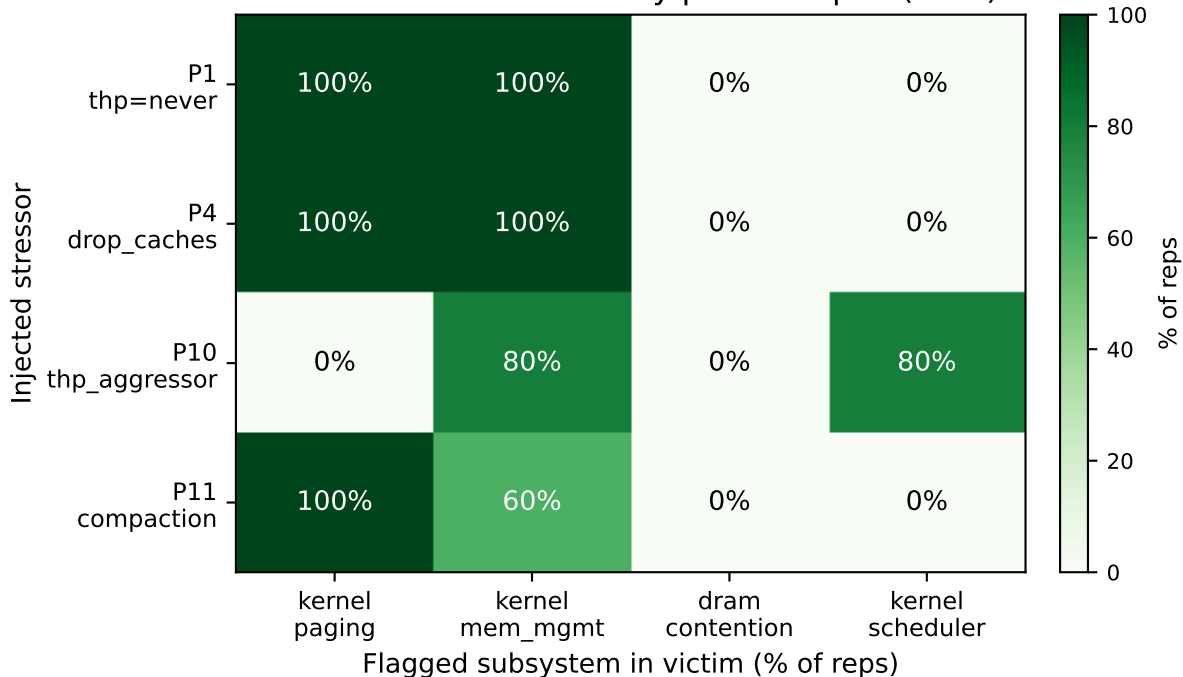
Victim-Mode vulnerability profile: sqlite (B0.5)
