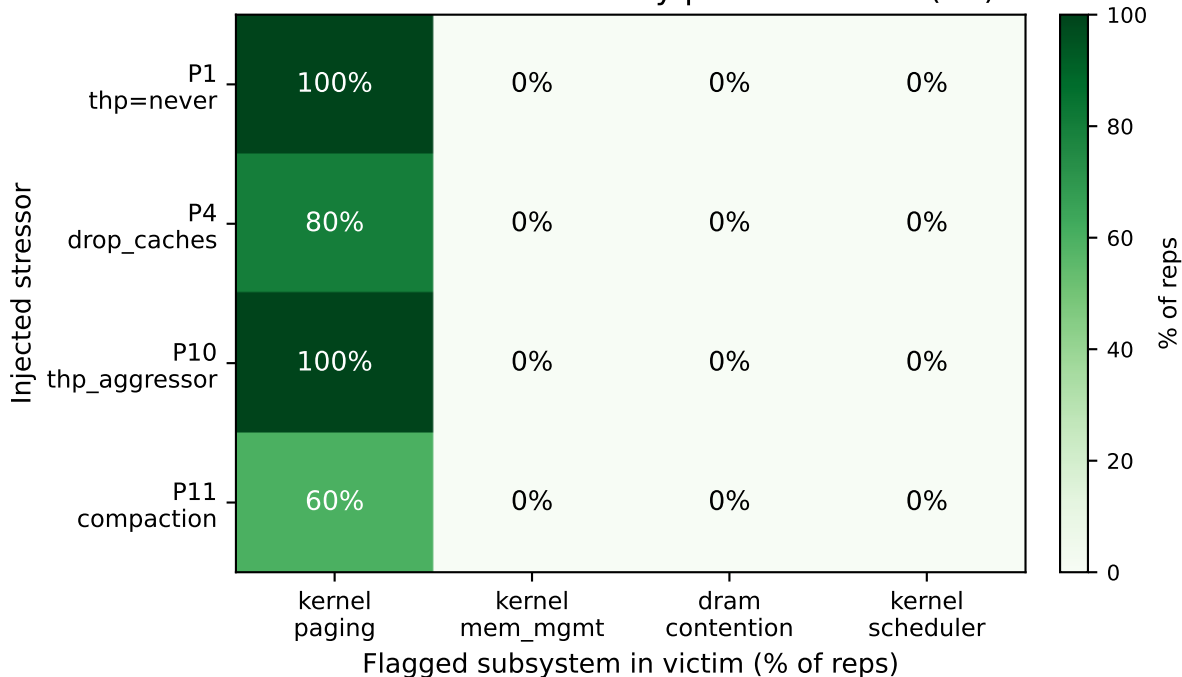
Victim-Mode vulnerability profile: stream (B2)
