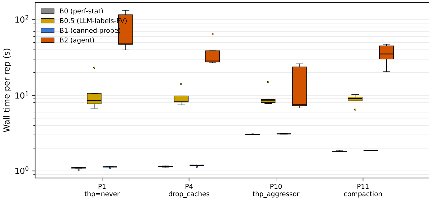
Time-to-diagnosis distribution (gups)
