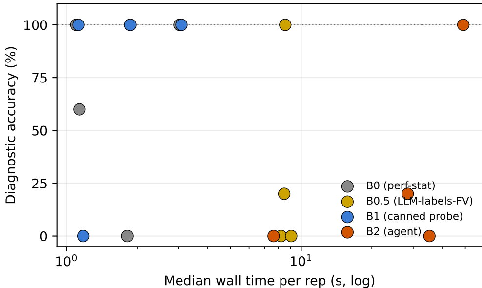
Accuracy vs latency (gups) each point = one (baseline, perturbation) cell
