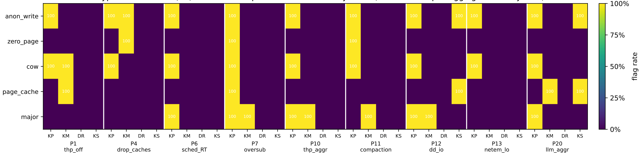
PF-type victim matrix (B0): 5 victims x 9 perturbations x 4 subsystems (cell = % of reps flagging that subsystem)
