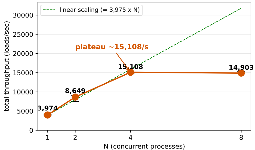
(b) total throughput plateaus
