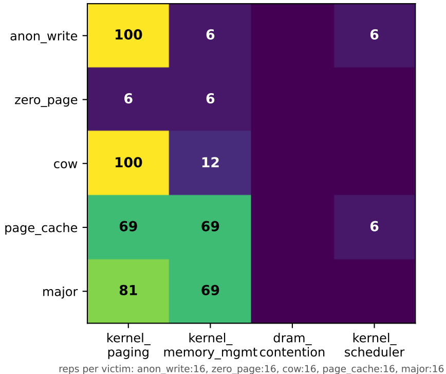
(a) B0 — rule-table
