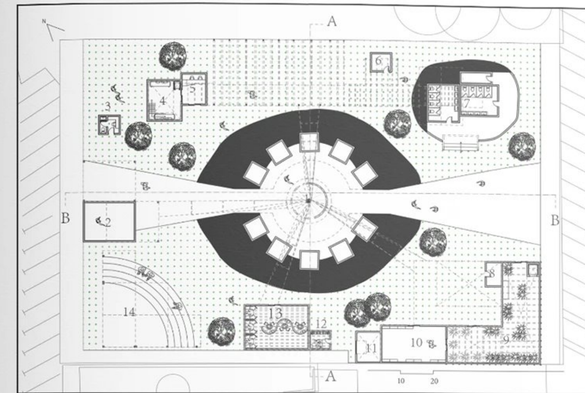
MOUND PARK - GROUND FLOOR PLAN Scale 1:200
