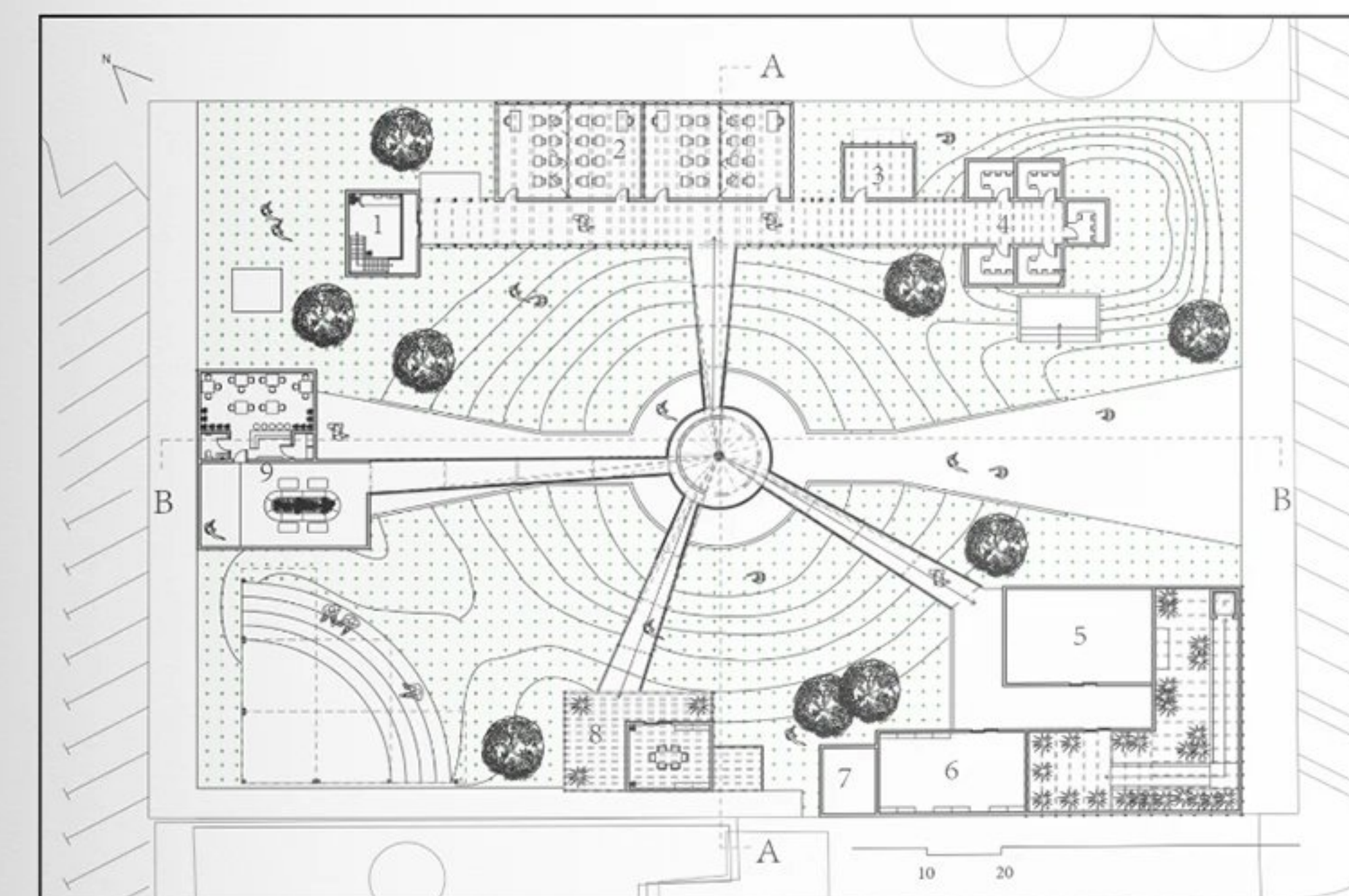
MOUND PARK - FIRST FLOOR PLAN Scale 1:200
