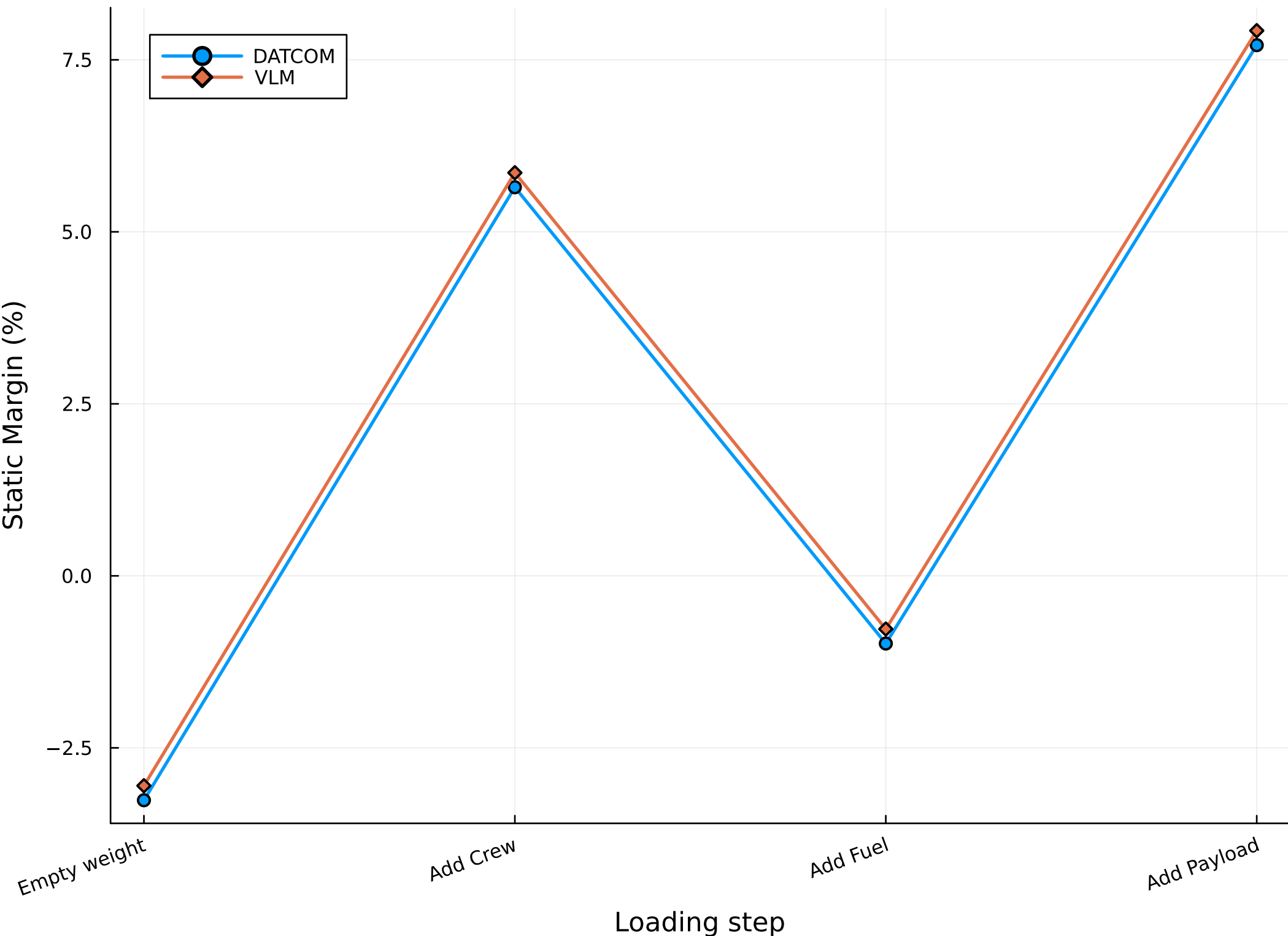
Static Margin During Representative Loading Cases
