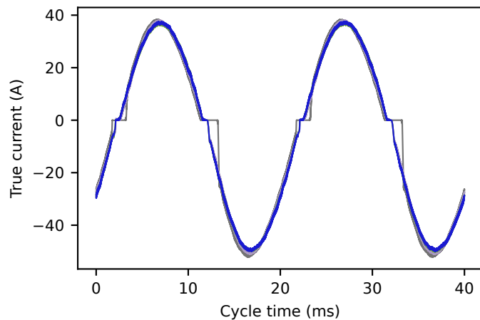
E-AC-02b: late-attack current
