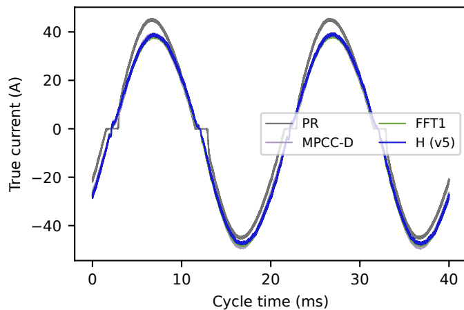
E-AC-01a: late-attack current
