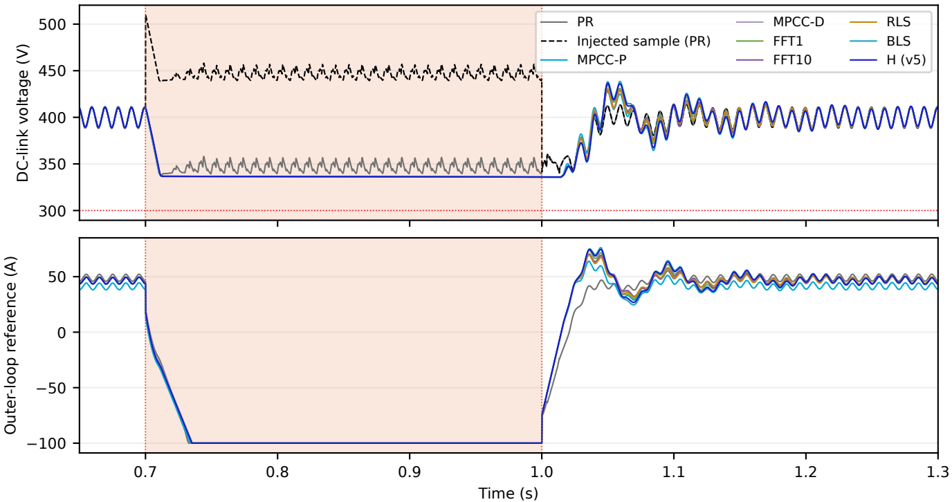
E-DC-01c: +100 V sensing bias; rectifier clamping and reference saturation
