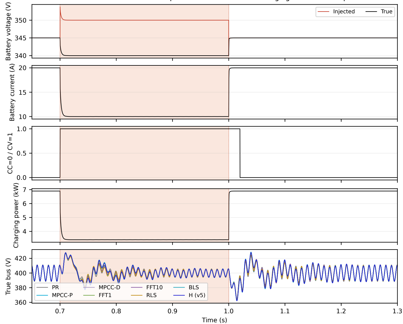
E-BAT-02b: +10 V bias → premature CV → 3.40 kW charging → PFC load step
