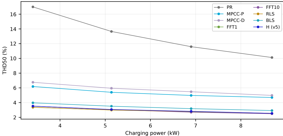
Current quality at attack-induced charging operating points
