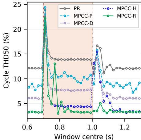
DC-link bias +50 V
