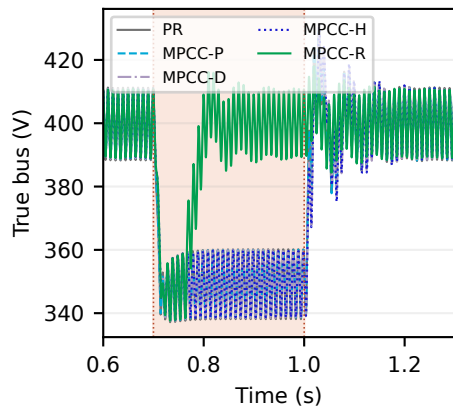
DC-link bias +50 V
