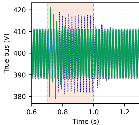
AC-voltage bias +34 V
