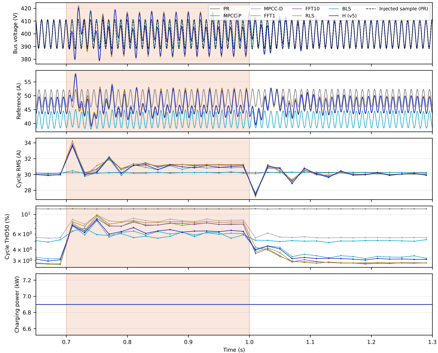
E-AC-01b: full unprotected phase-one state response (1 MHz cycle metrics)
