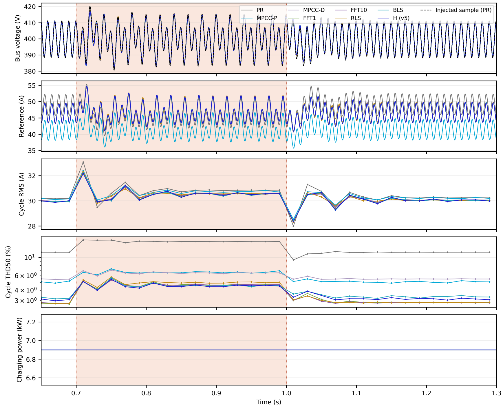
E-AC-02b: full unprotected phase-one state response (1 MHz cycle metrics)
