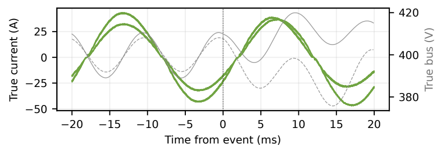
RLS
