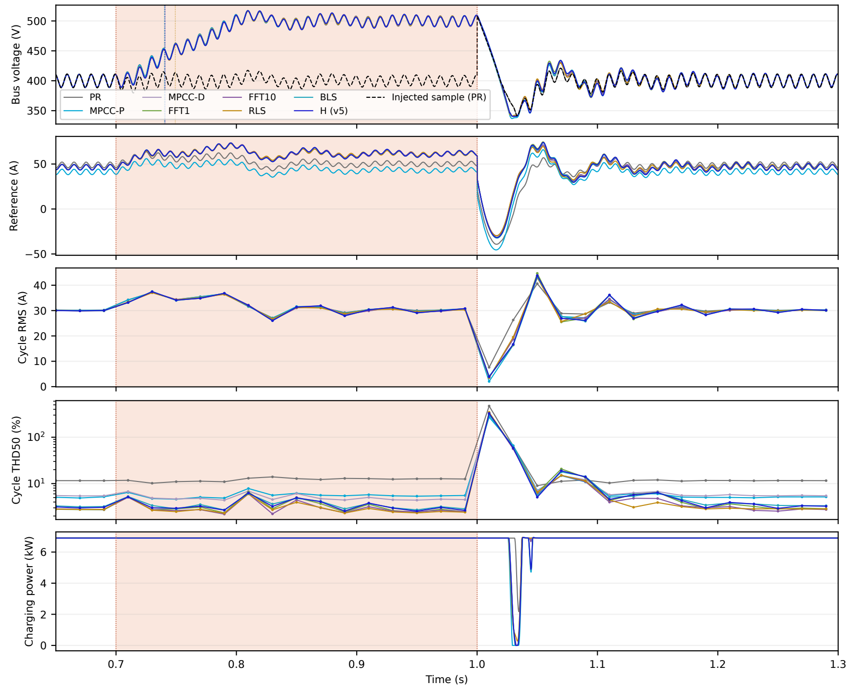
E-DC-02b: full unprotected phase-one state response (1 MHz cycle metrics)
