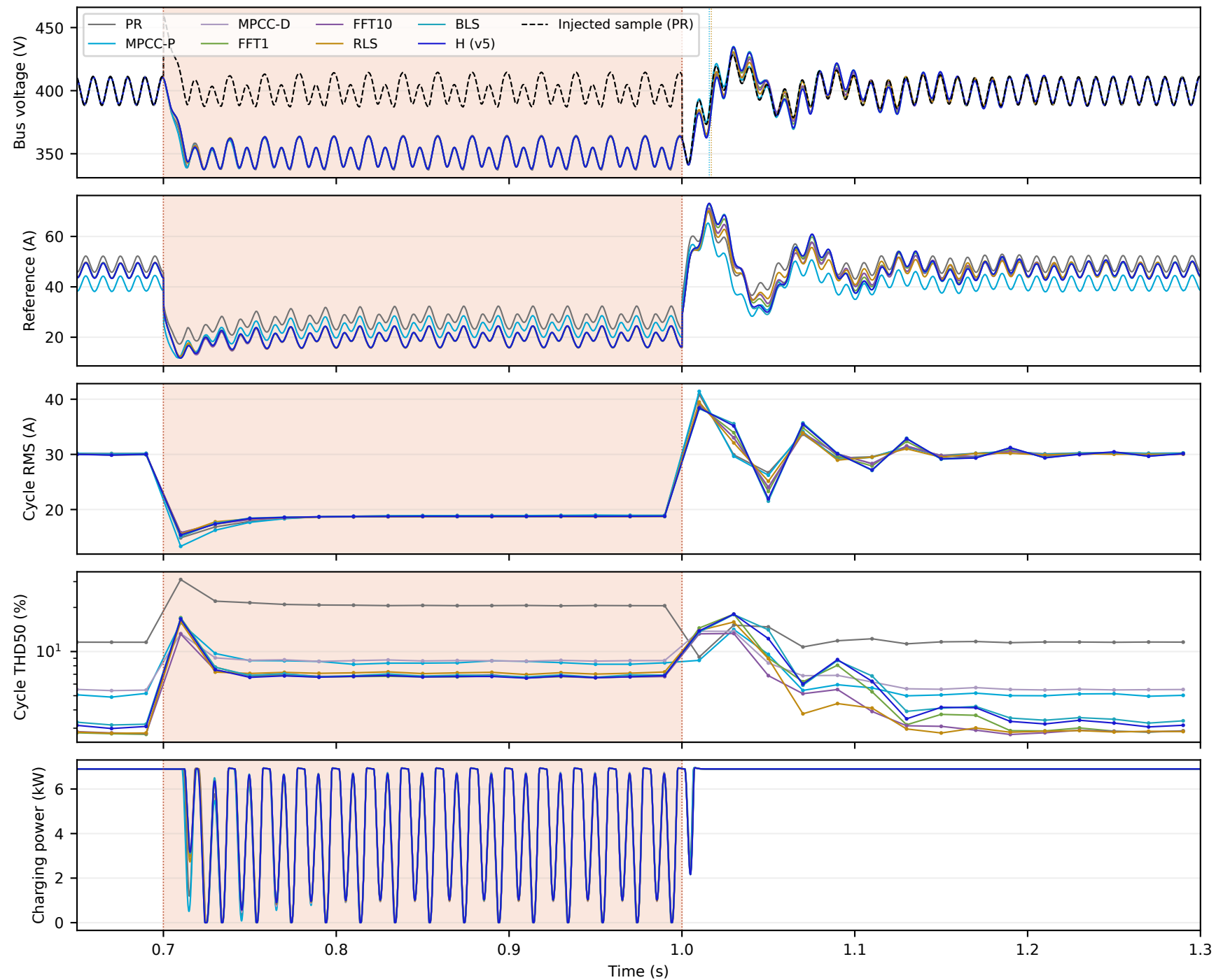
E-MUL-01: full unprotected phase-one state response (1 MHz cycle metrics)
