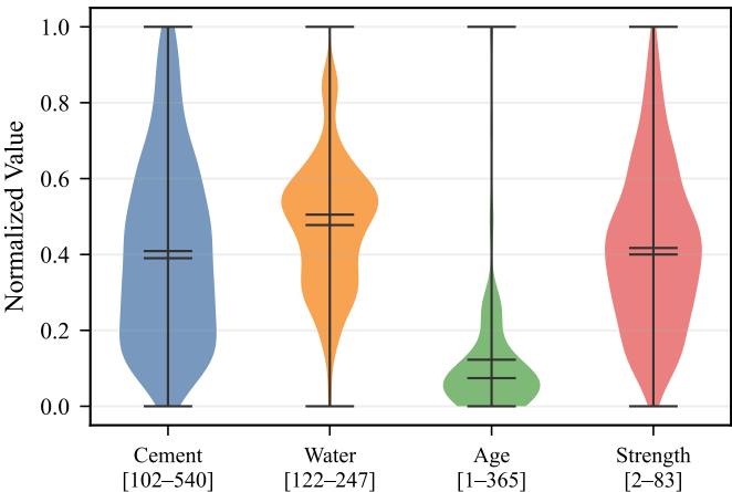
Violin Plots of Key Variables
