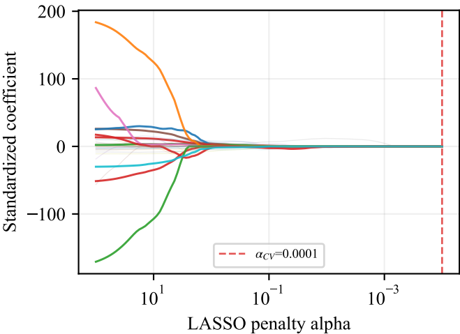
LASSO Coefficient Path
