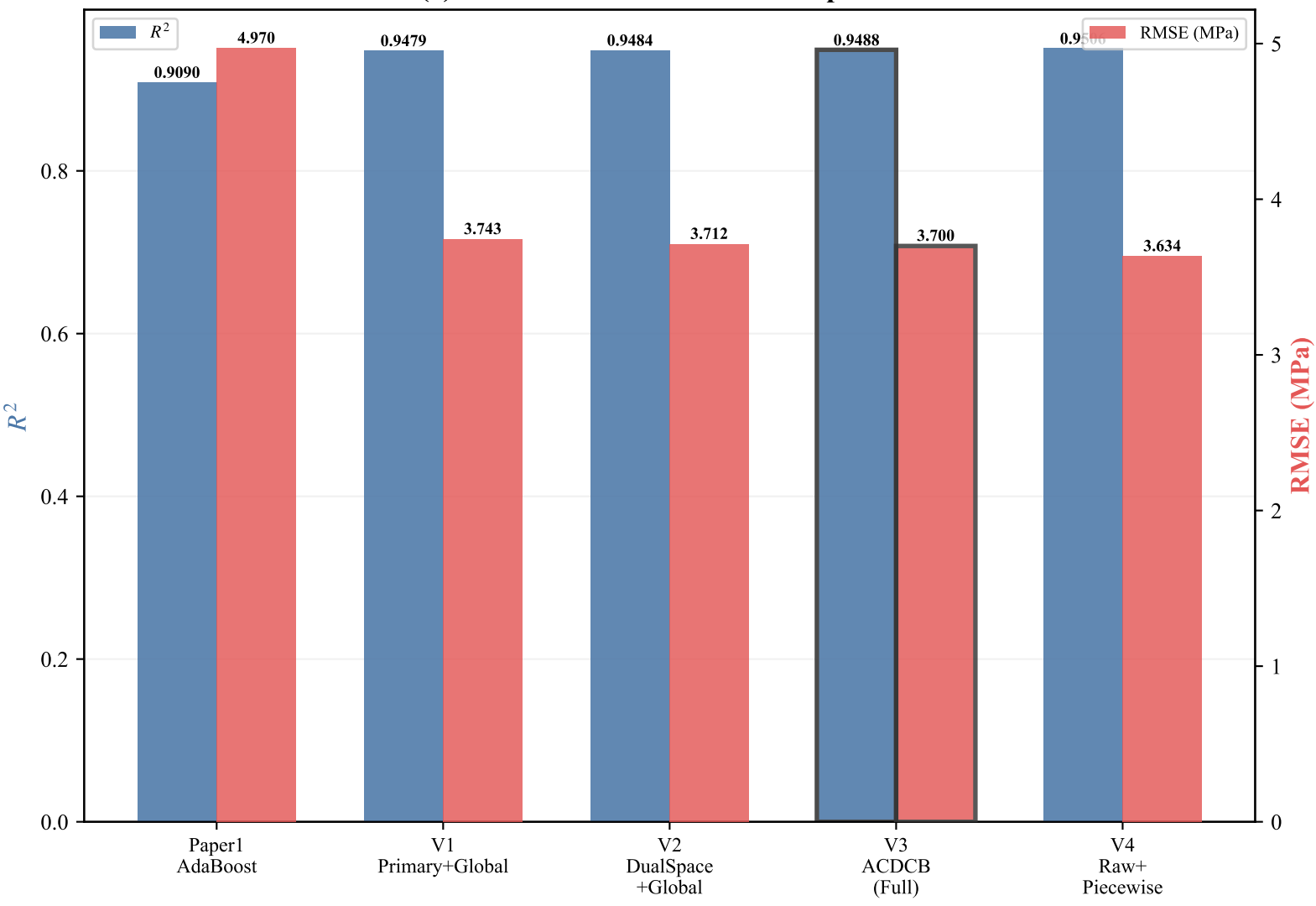
(a) Ablation: R^2 and RMSE Comparison
