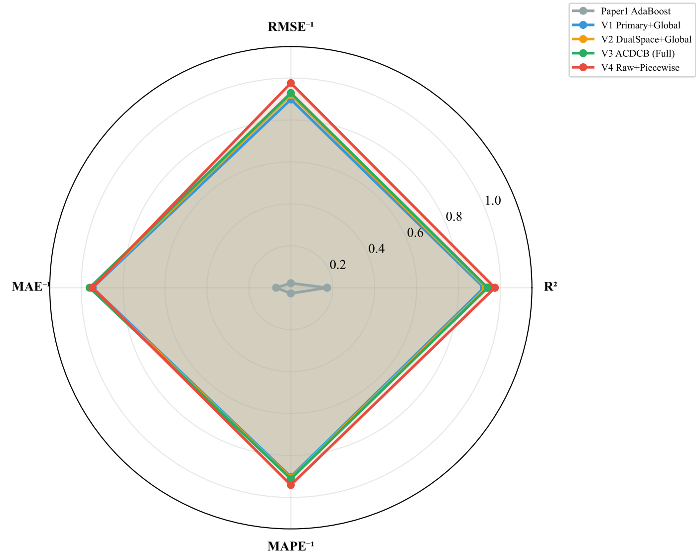
(b) Multi-Metric Radar Comparison
