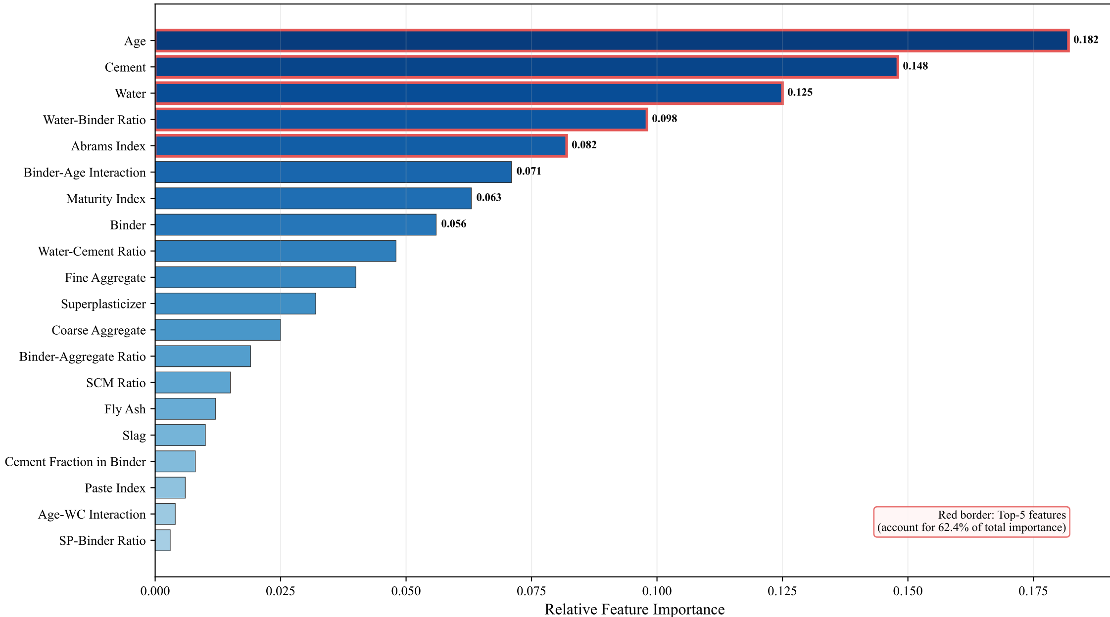
Feature Importance Ranking in ACDCB Ensemble
