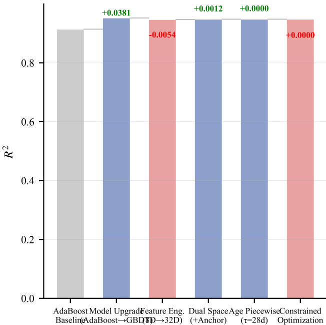
UCI ( N=1,030 )
