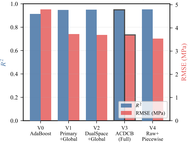
Ablation: R^2 and RMSE (10-fold)
