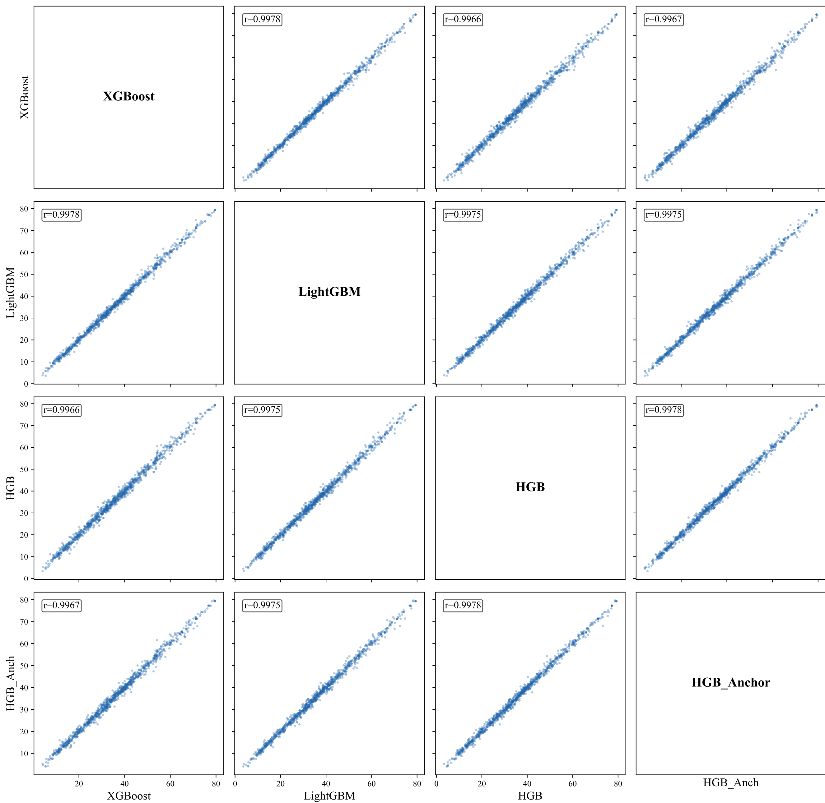
OOF Prediction Cross-Correlation Matrix
