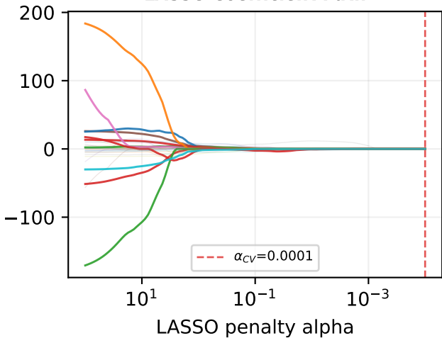
LASSO Coefficient Path
