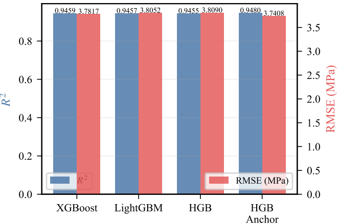
Single Model OOF Performance
