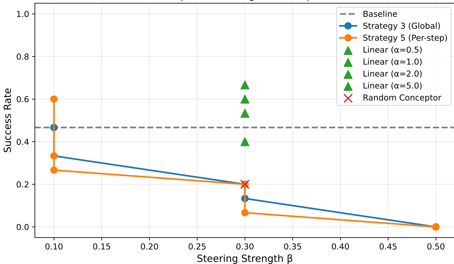
Conceptor Steering: handle-pull-v3
